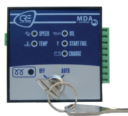
MDA MODULE FRONT FACE KEYSWITCH
