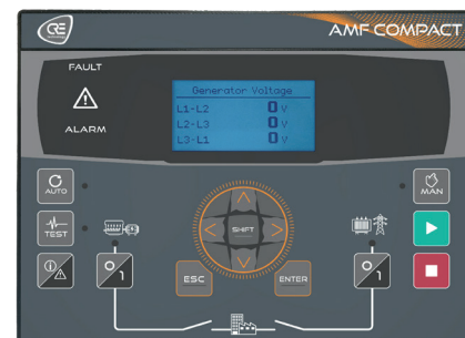
AMF COMPACT WITH DISPLAY
