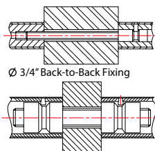
Ø 1-1/4" Back-to-Back Fixing
