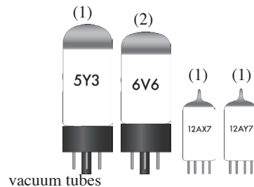
vacuum tubes
