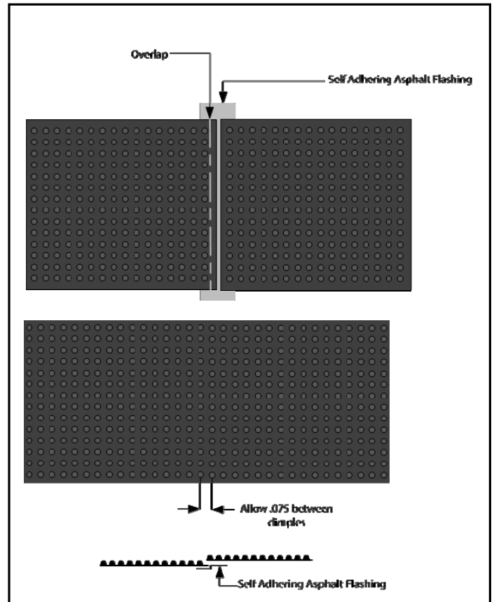
Pup-Drain Seaming Detail
