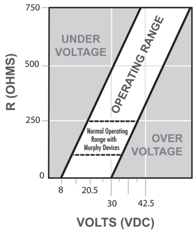
LOOP RESISTANCE GRAPH
